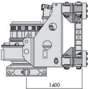
Drilling axis extension Slitta supplementare
