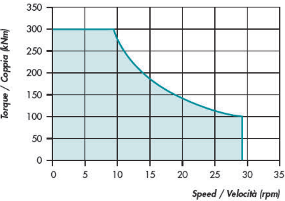
H30 ROTARY HEAD ROTARY H30
