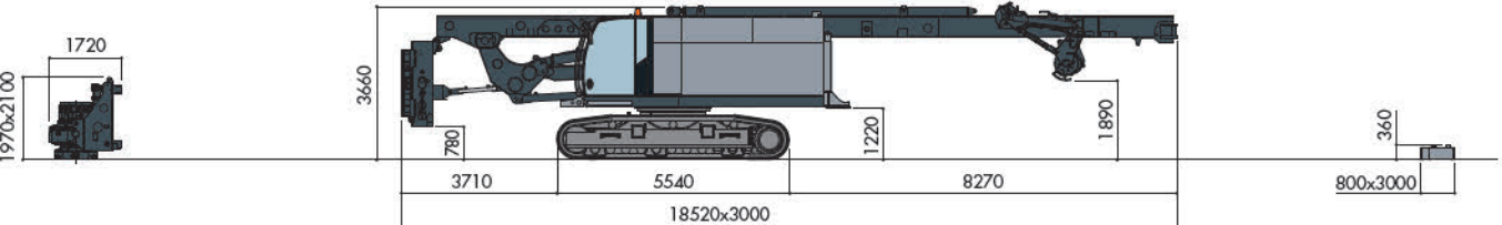
H30 rotary Rotary H26 ~ 6100 kg
