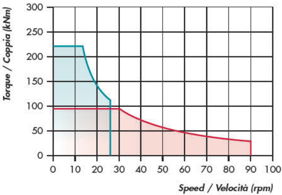
H30SX ROTARY HEAD ROTARY H30SX
