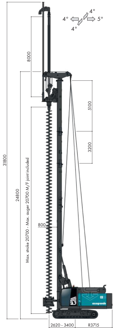
CFA ARRANGEMENT
