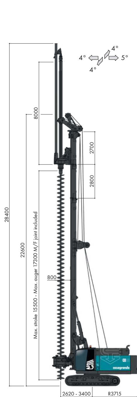
CFA-R ARRANGEMENT
