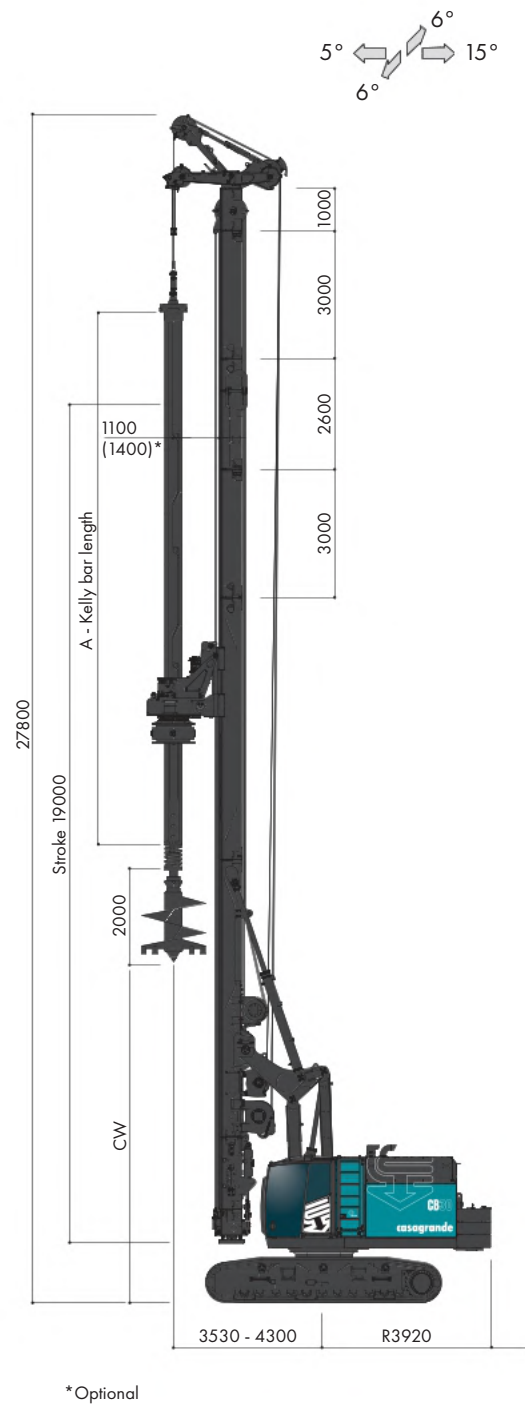
CROWD WINCH ARRANGEMENT
